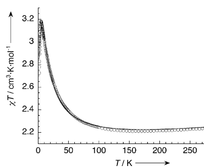
Fig. 2 Thermal dependence of \chi_{\text{M}}T for \text{I}^{2+} 2\text{PF}_6^- ; (○) experimental data; (—) fitting curve.
