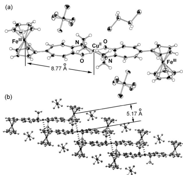
Fig. 1 X-ray structure of \text{I}^{2+} 2\text{PF}_6^- \text{C}_2\text{H}_4\text{Cl}_2 . (a) ORTEP drawing (50% probability). (b) Packing structure.
